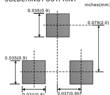
SOLDERING FOOTPRINT
