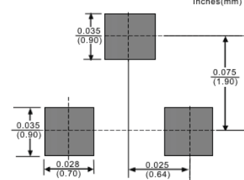
SOT-323 Recommended Footprint
