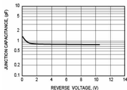
FIG. 3 - TYPICAL JUNCTION CAPACITANCE
