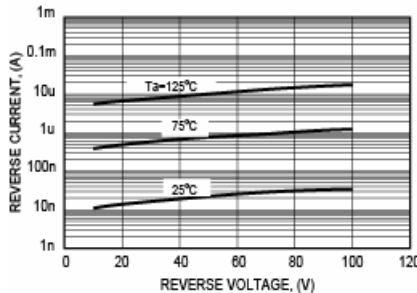
FIG. 2 - REVERSE CHARACTERISTICS
