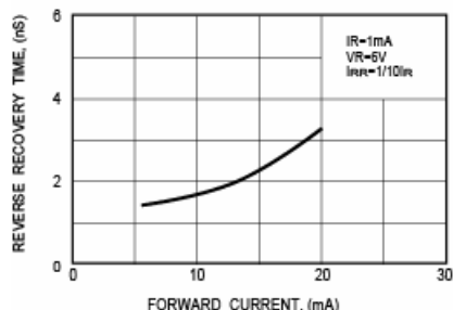
FIG. 4 - REVERSE RECOVERY TIME CHARACTERISTICS
