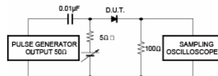
FIG. 6 - REVERSE RECOVERY TIME MEASUREMENT CIRCUIT
