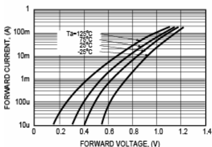
FIG. 1 - FORWARD CHARACTERISTICS
