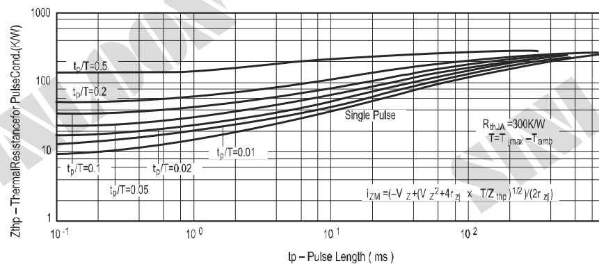
Fig 11. Thermal Response
