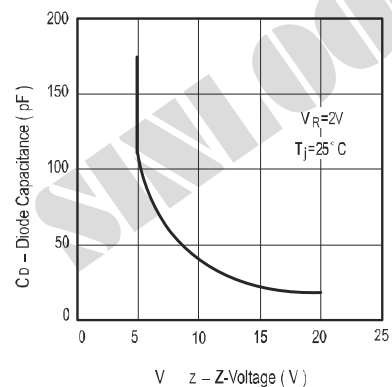
Fig 6. Diode Capacitance vs. V_Z -Voltage
