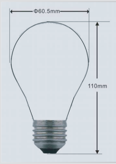
Lamp Dimensions
