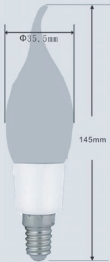
Lamp Dimensions
