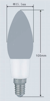
Lamp Dimensions
