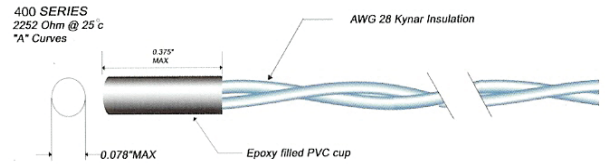
LS400 Series 2252 Ohms at 25°C "A" Curve
