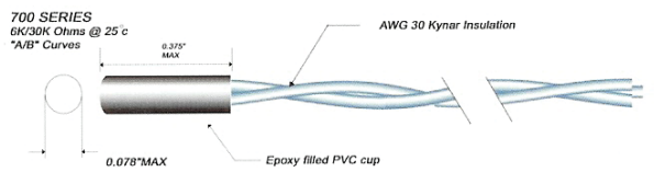
LS700 Series 6k/30k Ohms at 25°C "A" Curve
