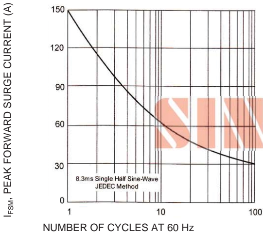
Fig-3 Maximum Non-Repetitive Peak FWD Surge Current
